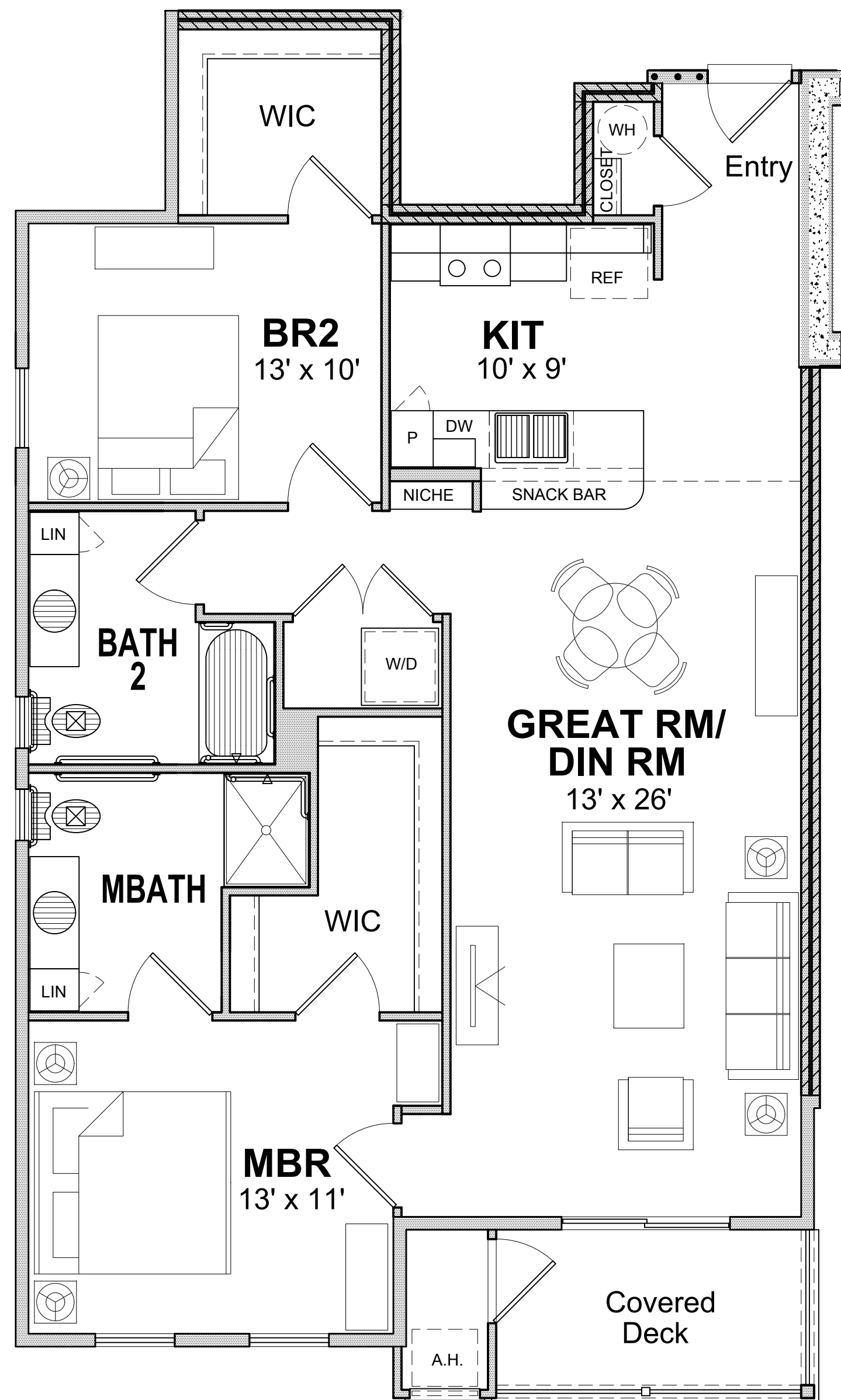
APARTMENT BUILDING - UNIT F 1185 SF (Two Bedroom, Two Bath)
