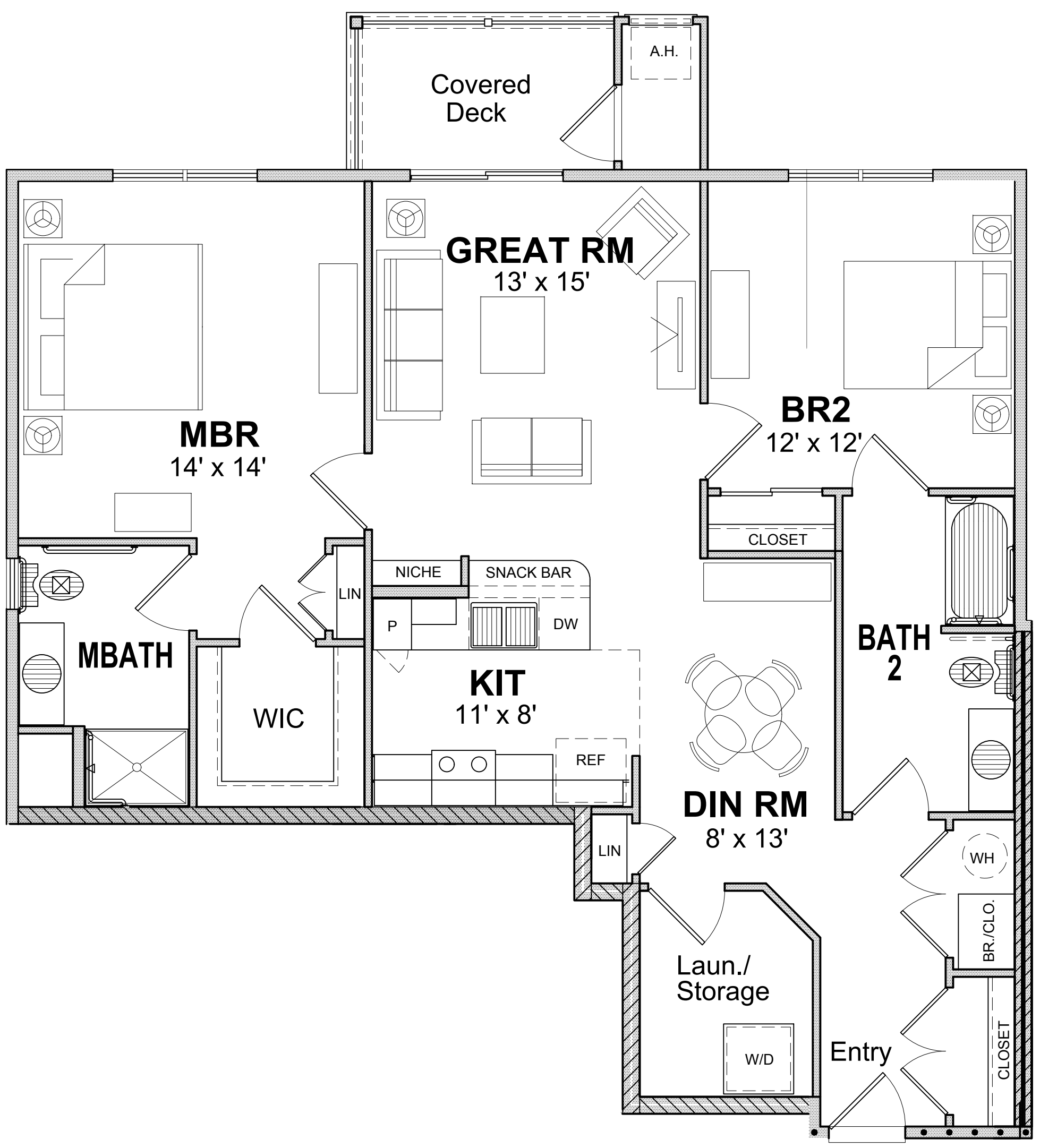
APARTMENT BUILDING - UNIT H 1205 SF (Two Bedroom, Two Bath)
