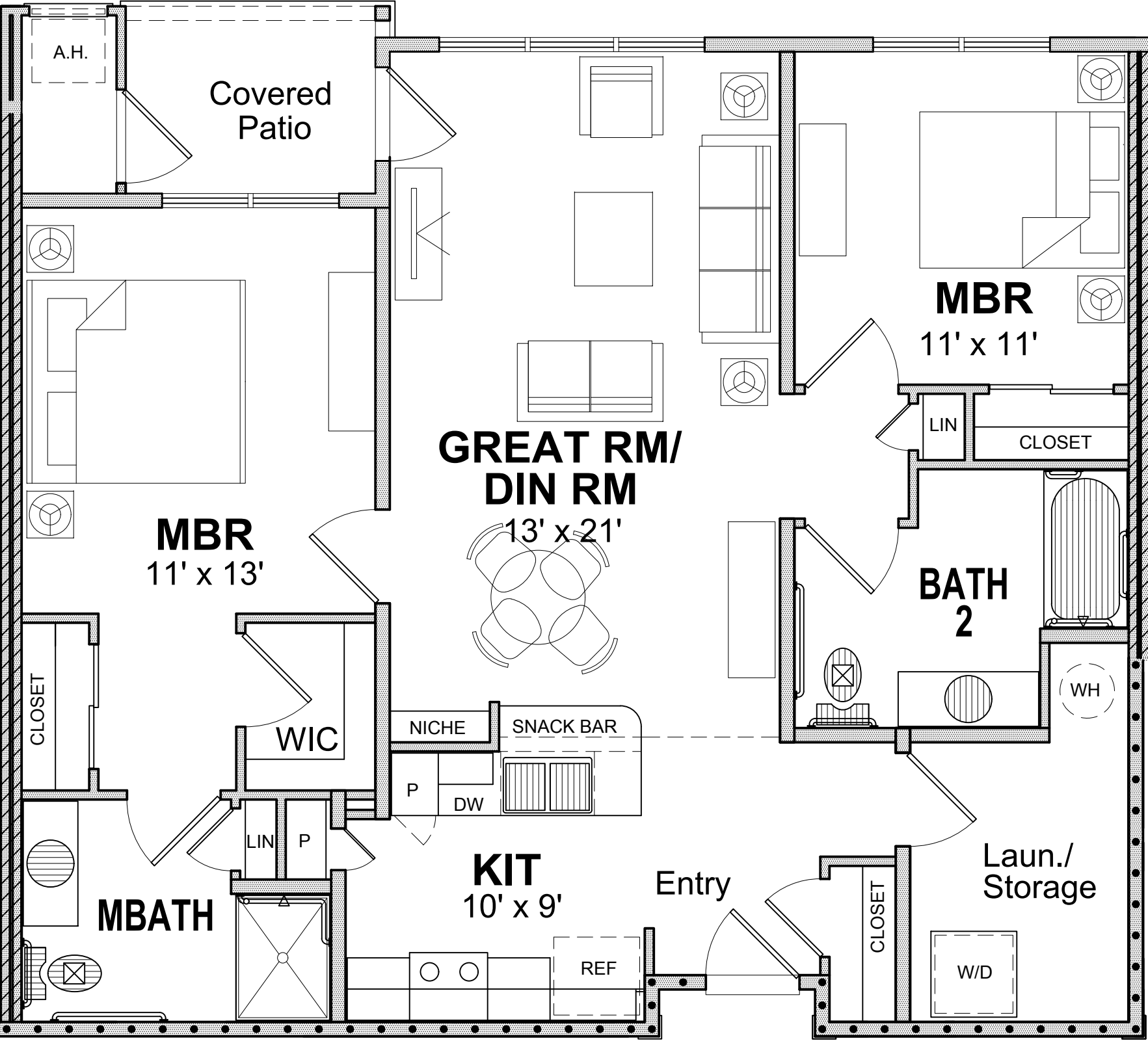
APARTMENT BUILDING - UNIT D 1100 SF (Two Bedroom, Two Bath)
