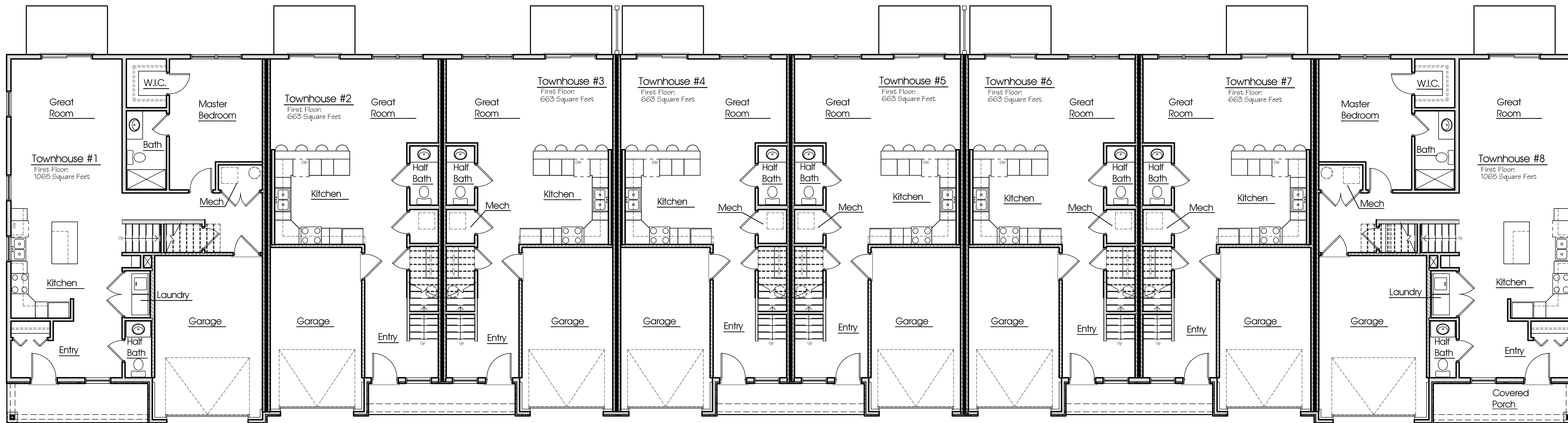
1st Floor Townhouse
